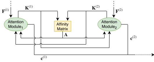
Fig. 6. An illustration of parallel co-attention.
