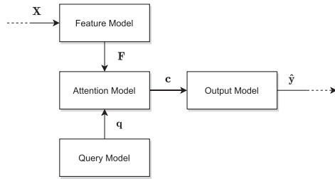
Fig. 1. An illustration of the general structure of the task model.
