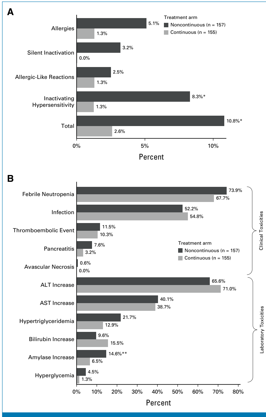
FIG 3. (A) Rate of hypersensitivity and (B) other clinical and laboratory toxicities (CTCAE ≥grade 3) after random assignment. Inactivating hypersensitivity reactions are the sum of allergies and silent inactivations. Hypersensitivity is the sum of allergies, silent inactivation, and allergic-like reactions. Rate of allergies, silent inactivations, and allergic-like reactions were not tested because of small numbers. * P < .01 ; ** P < .05 . CTCAE, Common Terminology Criteria for Adverse Events.
