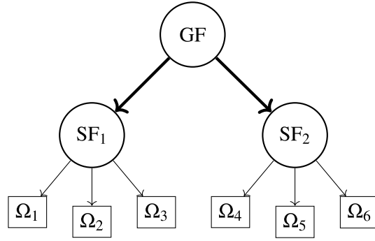
FIGURE 2. Example of second-order disjoint factor model
