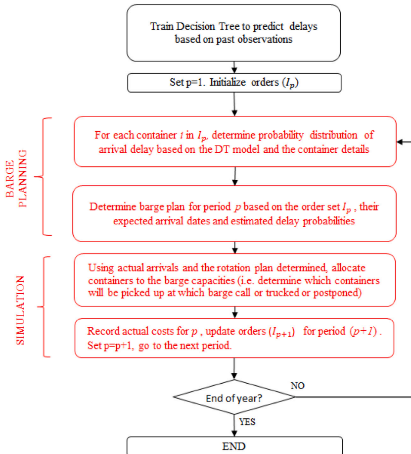
Fig. 2. The representation of the steps of the overall solution procedure. Source: Modified from Gumuskaya et al. (2020a).
