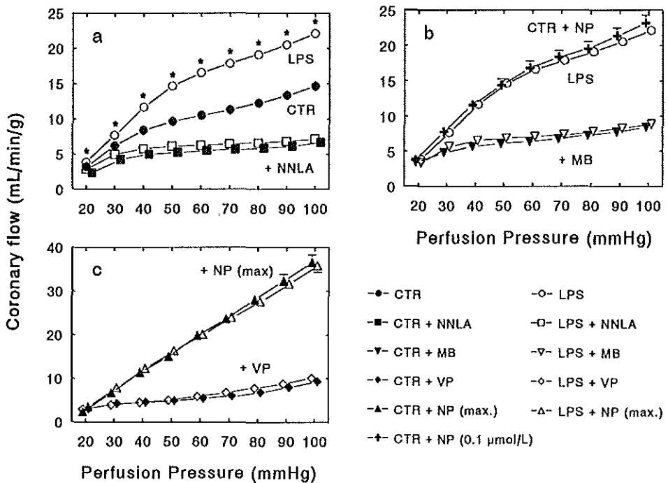
Figure 2. Line graphs showing effect of perfusion pressure on coronary flow in control and endotoxin-treated hearts with and without inhibition of the L-arginine/NO/cGMP pathway. (a) Coronary flow-pressure relations in ( n=15 ) control (CTR) (●) and ( n=16 ) endotoxin-treated (LPS) (○) hearts. Coronary flow following inhibition of NO-synthesis with 100 \mu\text{mol}/\text{L} N G -nitro-L-arginine (NNLA) in ( n=8 ) control (■) and ( n=8 ) endotoxin-treated (□) hearts. (b) Coronary flow following 5 \mu\text{mol}/\text{L} methylene blue (MB), an inhibitor of soluble guanylatecyclase, in ( n=4 ) control (▽) and ( n=4 ) endotoxin-treated (▽) hearts and coronary flow in ( n=4 ) untreated hearts with 0.1 \mu\text{mol}/\text{L} nitroprusside (NP) (⊕). (c) Coronary flow in a "passive" vascular bed following maximum vasodilatation with 10 \mu\text{mol}/\text{L} nitroprusside (NP) in ( n=5 ) control (▲) and ( n=5 ) endotoxin-treated (▲) hearts and with the direct smooth muscle constrictor vasopressin (VP) 1 nmol/L in ( n=4 ) control (◆) and ( n=4 ) endotoxin-treated (◆) hearts. Values are mean \pm SEM. * p<0.05 for LPS v. control.
