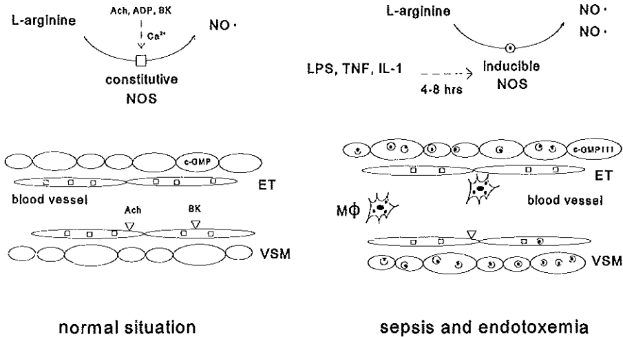
Figure 5. Schematic representation of blood vessels with the different types of NO synthase in the normal situation ( left ) and during sepsis and endotoxemia ( right ). In the normal situation only constitutive NO synthase is present in endothelial cells (ET) that can be stimulated by specific agonists such as acetylcholine (Ach), adenosinediphosphate (ADP), or bradykinine (BK) and/or flow induced shear stress. During sepsis and endotoxemia a second type of NO synthase is induced in macrophages (MΦ) and vascular smooth muscle cells (VSM) by stimulation with cytokines e.g., interleukin-1 (IL-1) and tumor necrosis factor (TNF), and endotoxin (LPS) with a lag-phase of 4-8 hours. This non-regulated inducible NO synthase produces large amounts of NO for long periods of time resulting in massive vasodilation and tissue damage.
