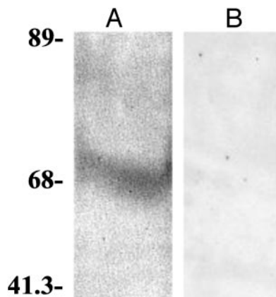
FIG. 2. Immunoblot of glycoproteins derived from a human corticotroph pituitary tumor with D_2 receptor antibody. A and B, Corticotroph pituitary tumor without (A) and with (B) preincubation of the antibody with the antigen. The specificity of the immunoblot is demonstrated by the complete disappearance of the signal after preincubation of the antibody with the antigen ( D_2 receptor peptide).
