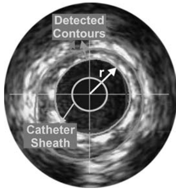
Figure 3. The increased propagation speed of the ultrasound signal crossing the catheter sheath was neglected in the BSC 30 MHz Ultracross ® software in the Clearview ® instrument. This must be taken into account for accurate radial, and thus also area measurements. Applying Equation 1 can retrospectively do this.
