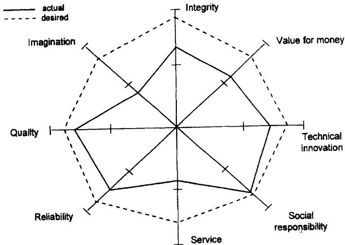
Figure 2: Cobweb Method
