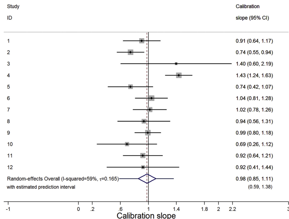
Fig. 2. Forest plot showing the calibration slope result from the trivariate random-effects meta-analysis (Table 1) for the DVT prediction model implemented using strategy (2).
