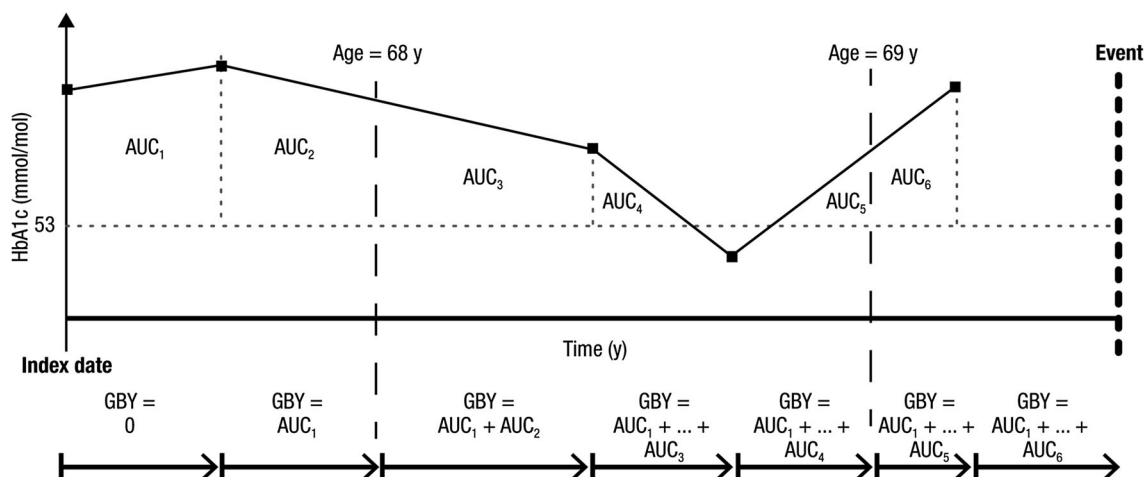
Fig. 1 Calculation of GBYs. AUC area under the curve, GBY glycemic burden year
