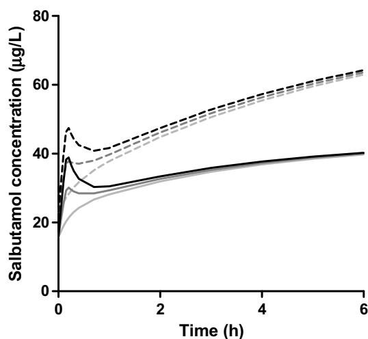
Fig. 3 Simulation of R-salbutamol (solid lines) and S-salbutamol (dotted lines) concentrations for a child weighing 15 kg, after a continuous intravenous salbutamol infusion of 0.5 \mu\text{g/kg/min} without a loading dose (light grey), or after a loading dose of 1.0 \mu\text{g/kg/min} (dark grey) or 1.5 \mu\text{g/kg/min} (black) over 10 min. The initial concentration before infusion is almost 20 \mu\text{g/L} as a result of salbutamol inhalation
