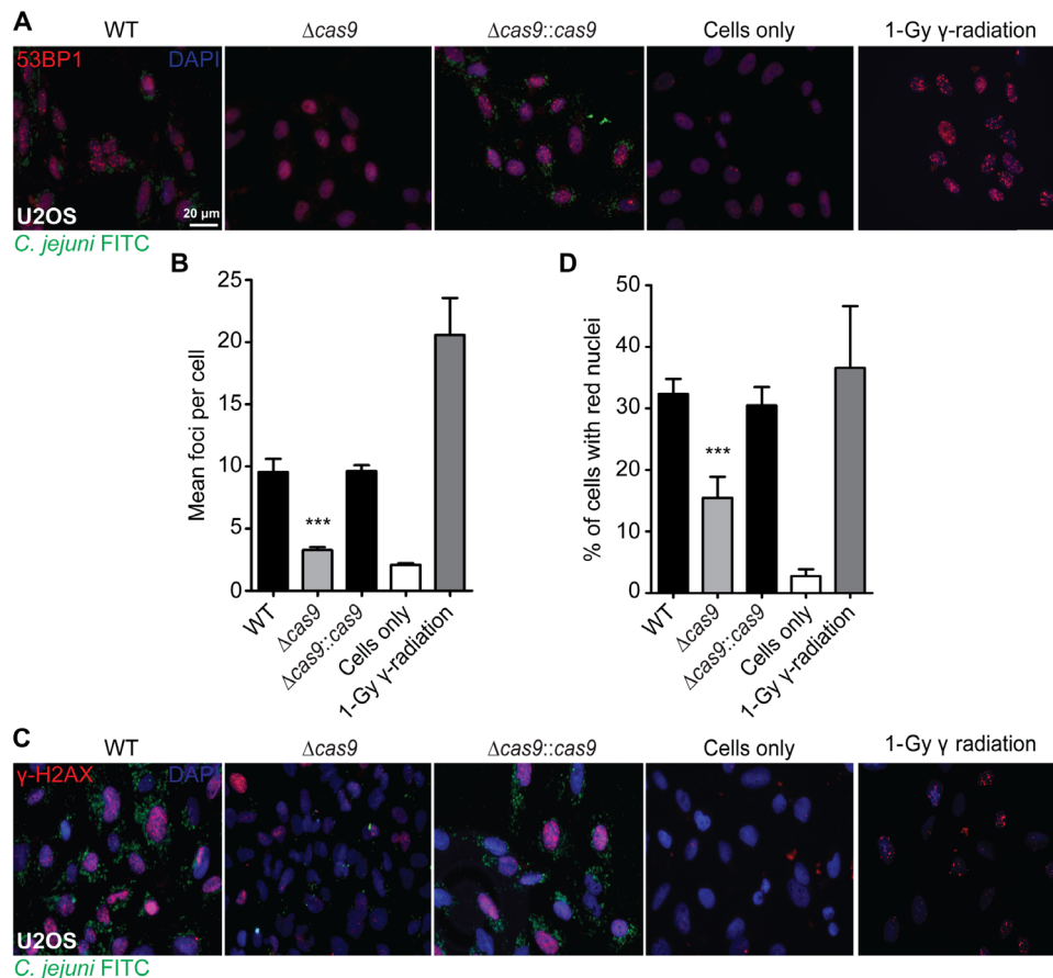
Fig. 2. CjeCas9 activates the chromatin and DNA integrity markers, 53BP1 and \gamma -H2AX, in U2OS cells. C. jejuni GB11 (WT) and its variants \Delta cas9 or \Delta cas9::cas9 were stained with anti- C. jejuni FITC (green), and nuclei were counterstained with DAPI (blue). Gamma ( \gamma )-irradiated cells are used as a positive control, and untreated cells were used as a negative control. (A) Representative microscopic images of human cells infected with WT, \Delta cas9 , or \Delta cas9::cas9 were stained for 53BP1 (red). (B) The number of 53BP1 related foci per cell (mean foci per cell, y axis) were counted in human cells. The C. jejuni bacteria used are shown on the x axis. (C) Representative microscopic images of human cells infected with WT, \Delta cas9 , or \Delta cas9::cas9 were stained for \gamma -H2AX (red). (D) The percentage of human cells with bright red nuclei is displayed on the y axis. The C. jejuni bacteria used are listed at the x axis. Values represent means \pm SEM. *** P < 0.001 [one-way analysis of variance (ANOVA), Bonferroni's multiple comparison test].
