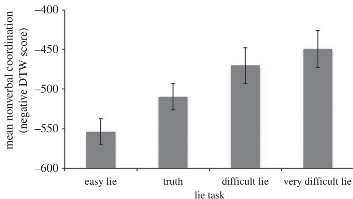
Figure 1. Mean nonverbal coordination (DTW) as a function of task. Error bars are 95% CI.
