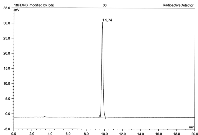
Figure 1. HPLC radiochromatogram of [ 18 F] 12 .
