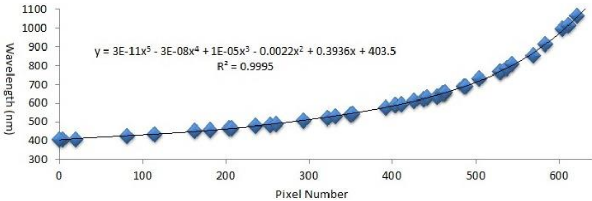
Figure 5. The trendline for calibration of the spectrometer with high R-squared value. The horizontal axis represents the pixel number and the vertical axis represents wavelength in nm.
