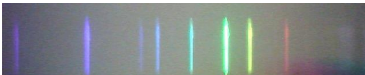
Figure 4. Lines of the Mercury lamps on the webcam sensor (360-1100 nm).
